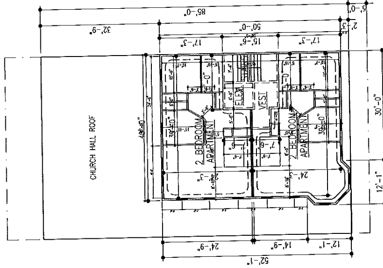
2nd & 3rd FLOOR PLAN
