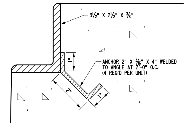
DETAIL "E"
