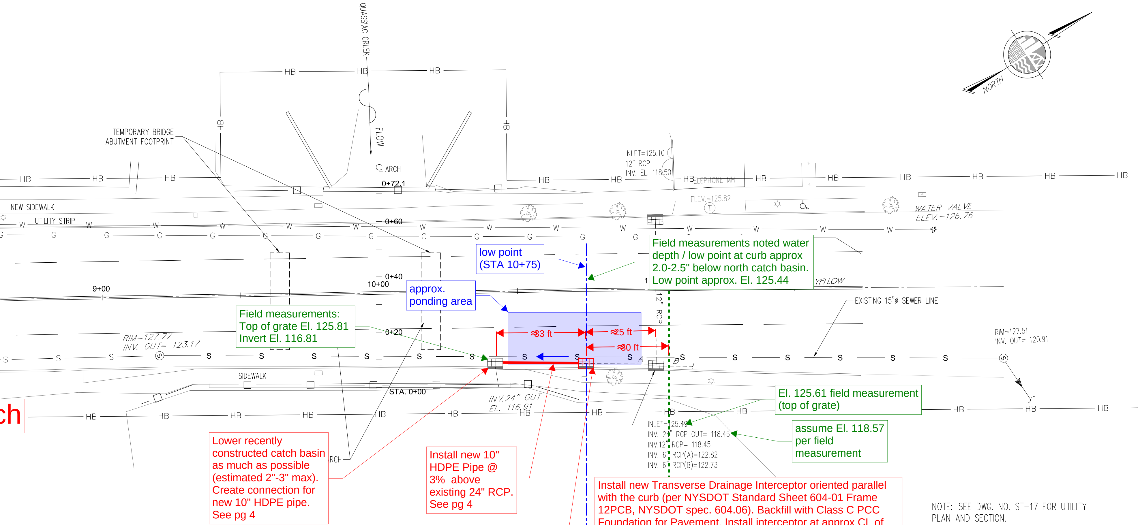
EXISTING/PROPOSED ROADWAY PLAN
