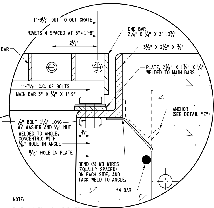
DETAIL "D"
