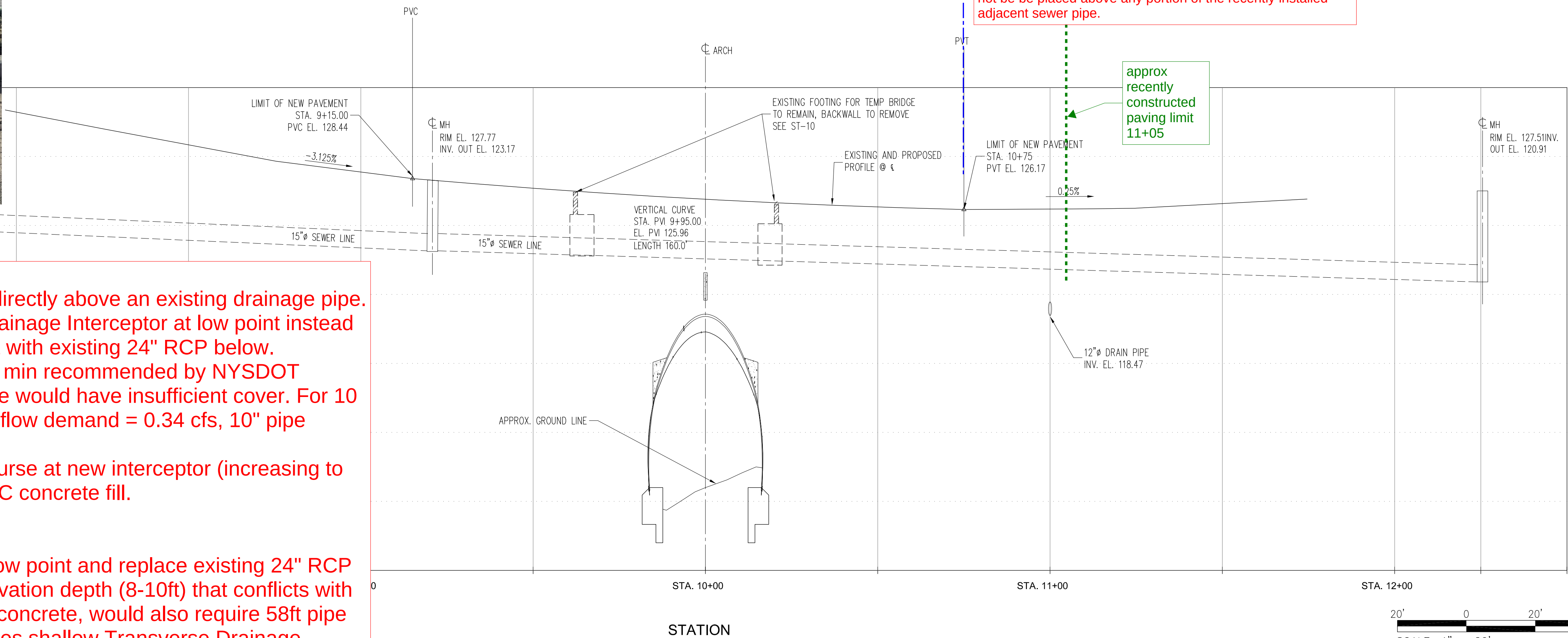
EXISTING/PROPOSED ROADWAY PROFILE
