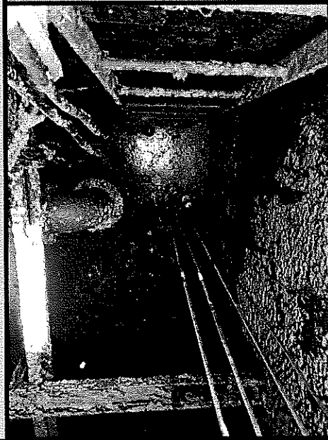
INSTALLED NEW FLOATS AT CRESCENT AVENUE PUMP STATION
