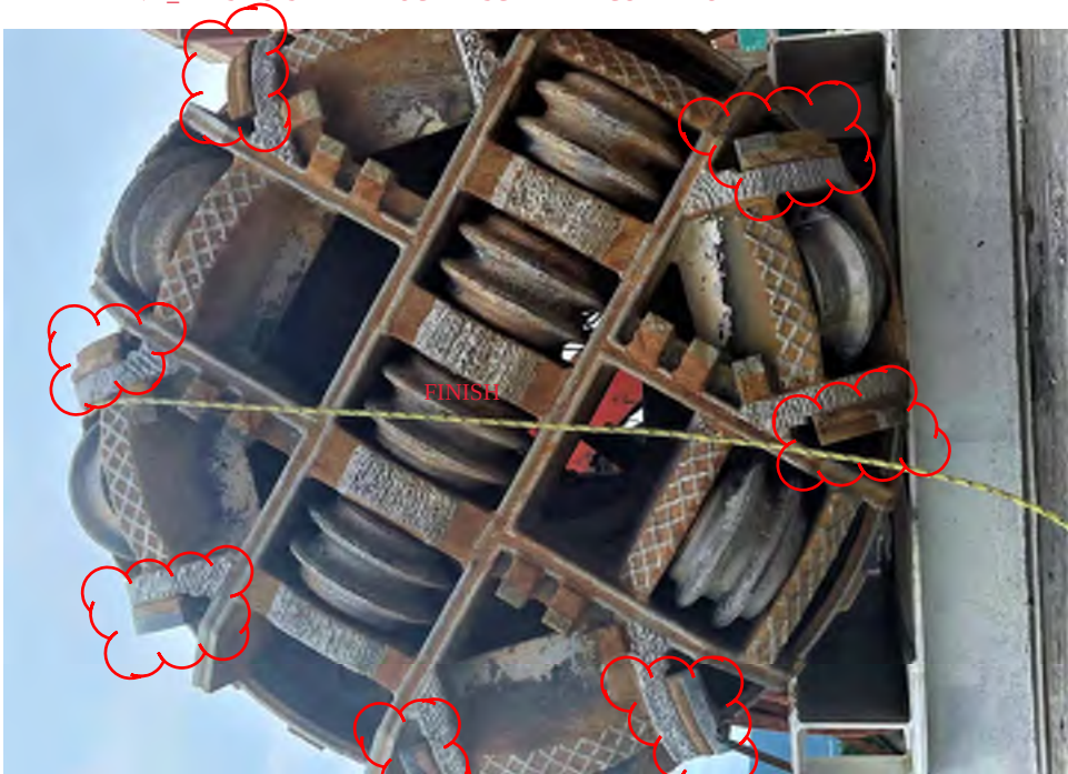
L2 - MT DRIVE_FINISH & START - BUCKET SCRAPER CONDITION
