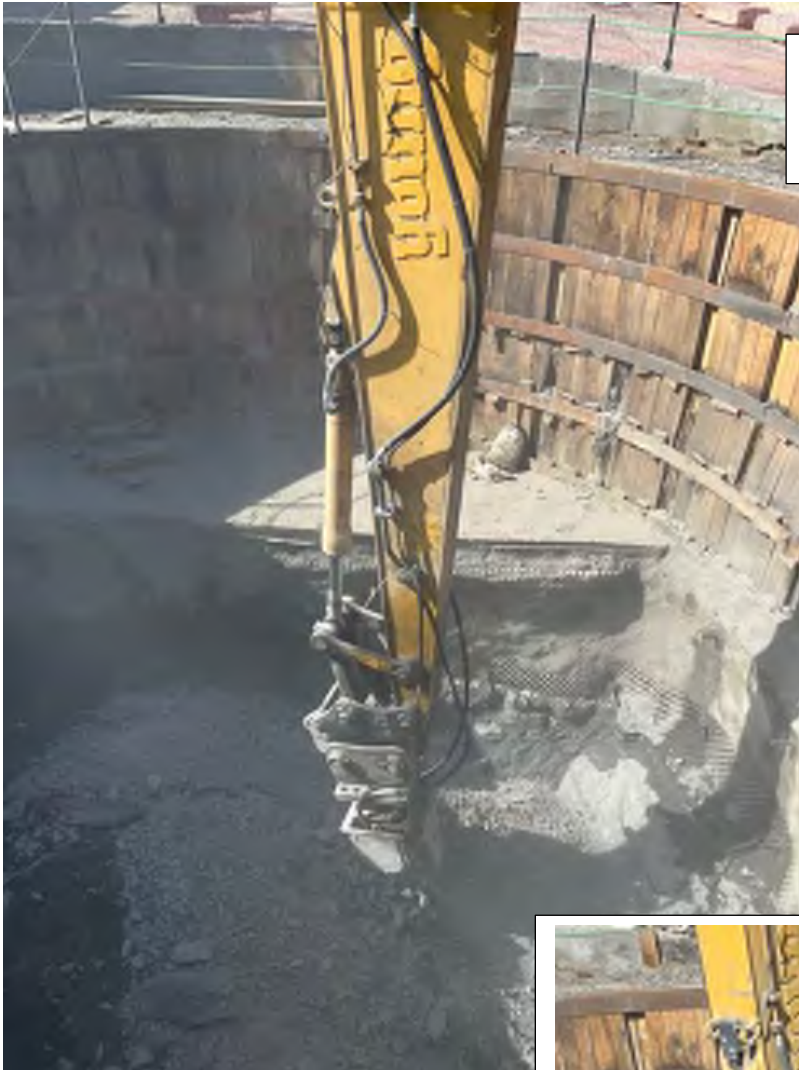
Photo 1 and 2 – Shaft 2138 during rock excavation.
