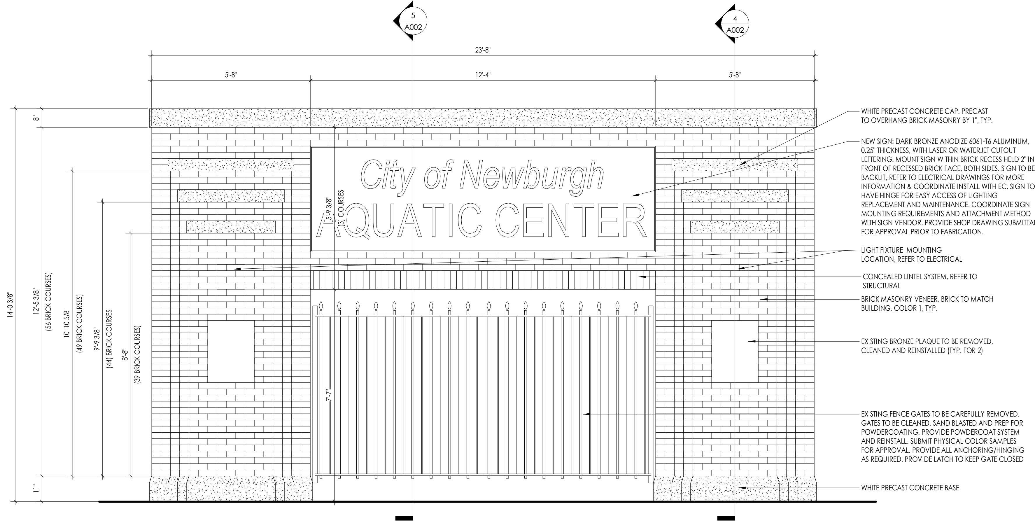
2 BRICK ARCH ELEVATION - STREET SIDE 1/2" = 1'-0"
