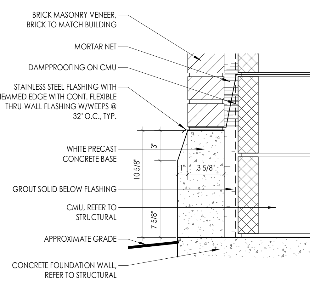
6 BASE OF WALL DETAIL - ARCH 1:6
