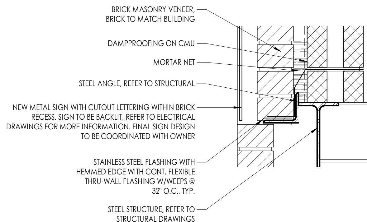
7 DETAIL @ BASE OF RECESS 1:6
