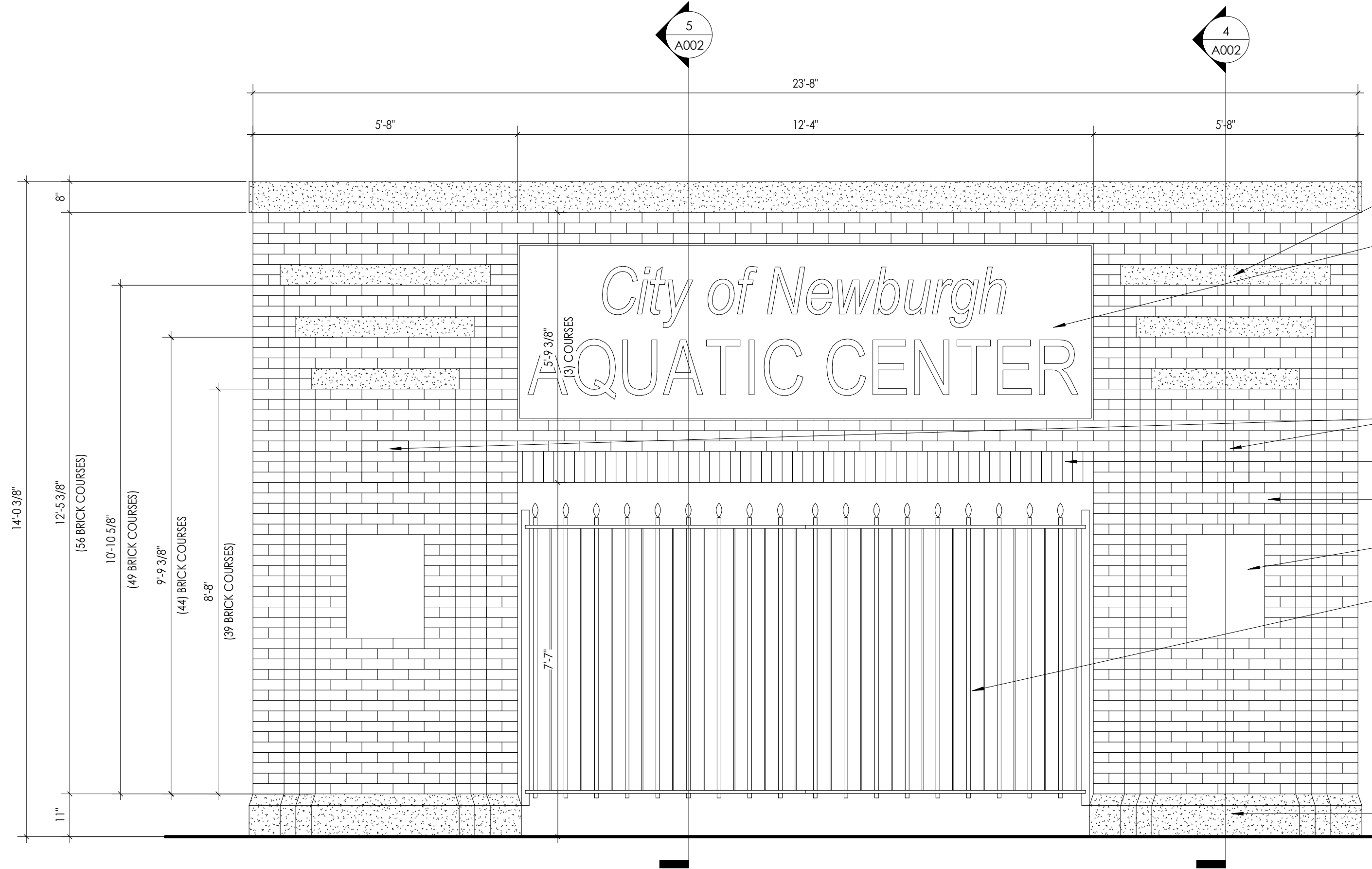
2 BRICK ARCH ELEVATION - STREET SIDE 1/2" = 1'-0"
