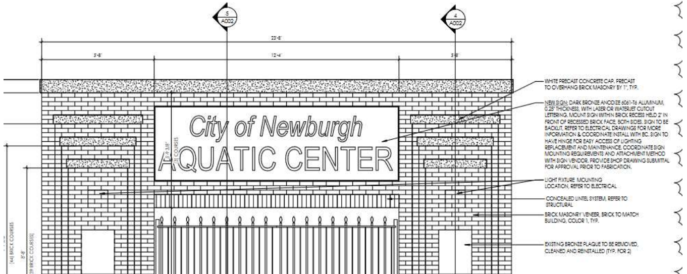
3 A002 BRICK ARCH ELEVATION - POOL SIDE 1/2" = 1'-0"
