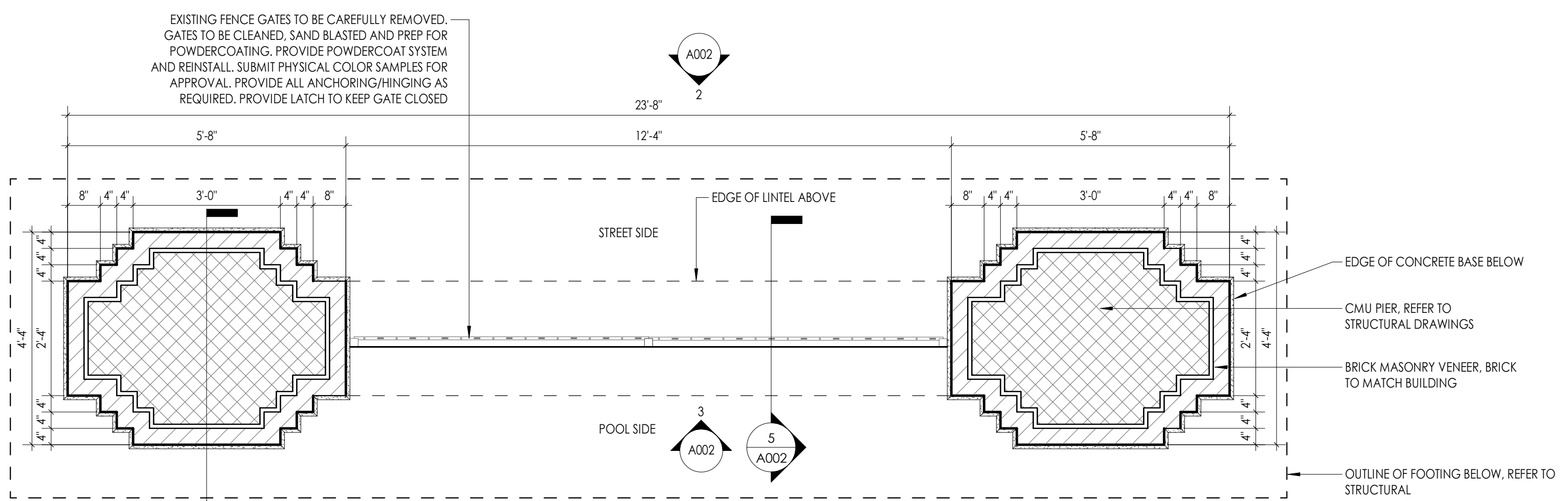
1 BRICK ARCH PLAN 1/2" = 1'-0"
