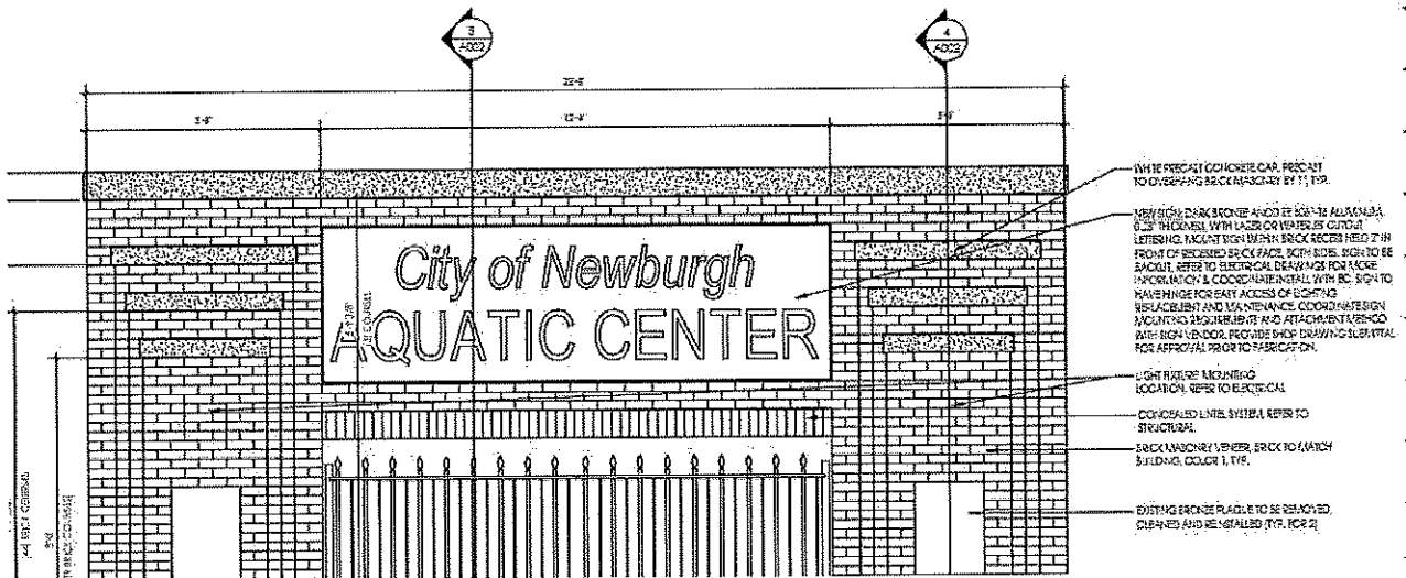
d BRICK ARCH ELEVATION - POOL SIDE A002 1/2" = 1'-0"
