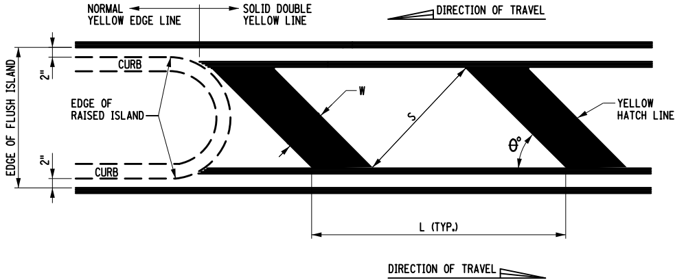
TYPICAL CROSS HATCH LINE DETAIL AT FLUSH OR RAISED ISLANDS AND AT MEDIAN AREAS
